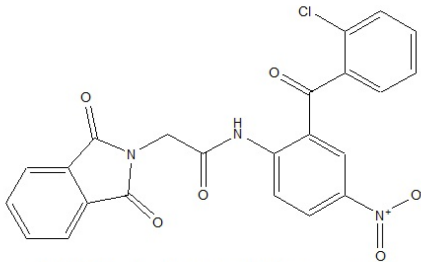
2-Phthalimidoacetamido-5-nitro-2'-chloro-benzophenone
