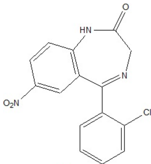
Clonazepam
